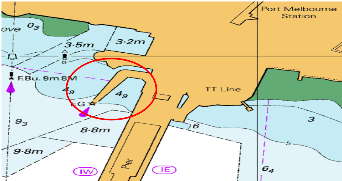
Figure 1 Finger Pier
